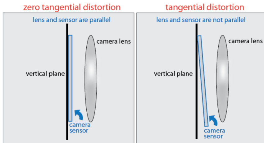
Figure 7: Tangential Distortion [35]
